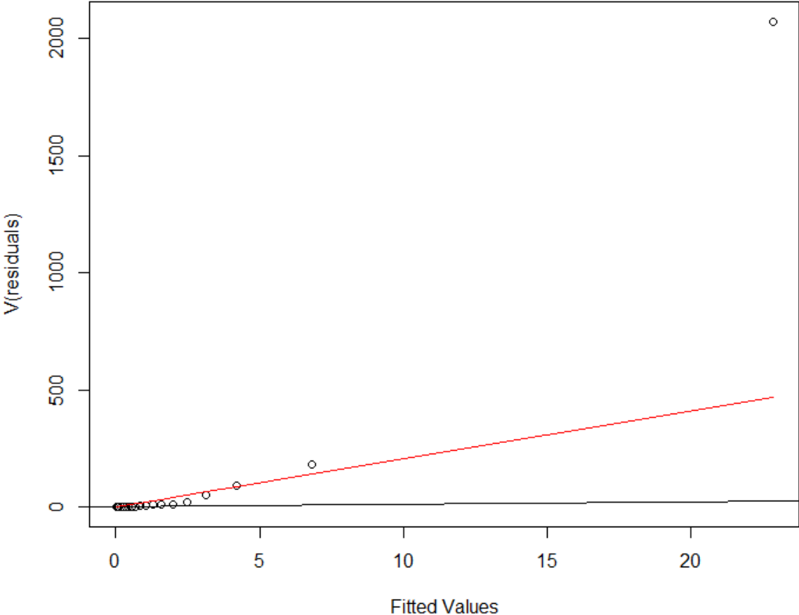
Figure 22: Mean-variance plot for best fitting guillemot model.
