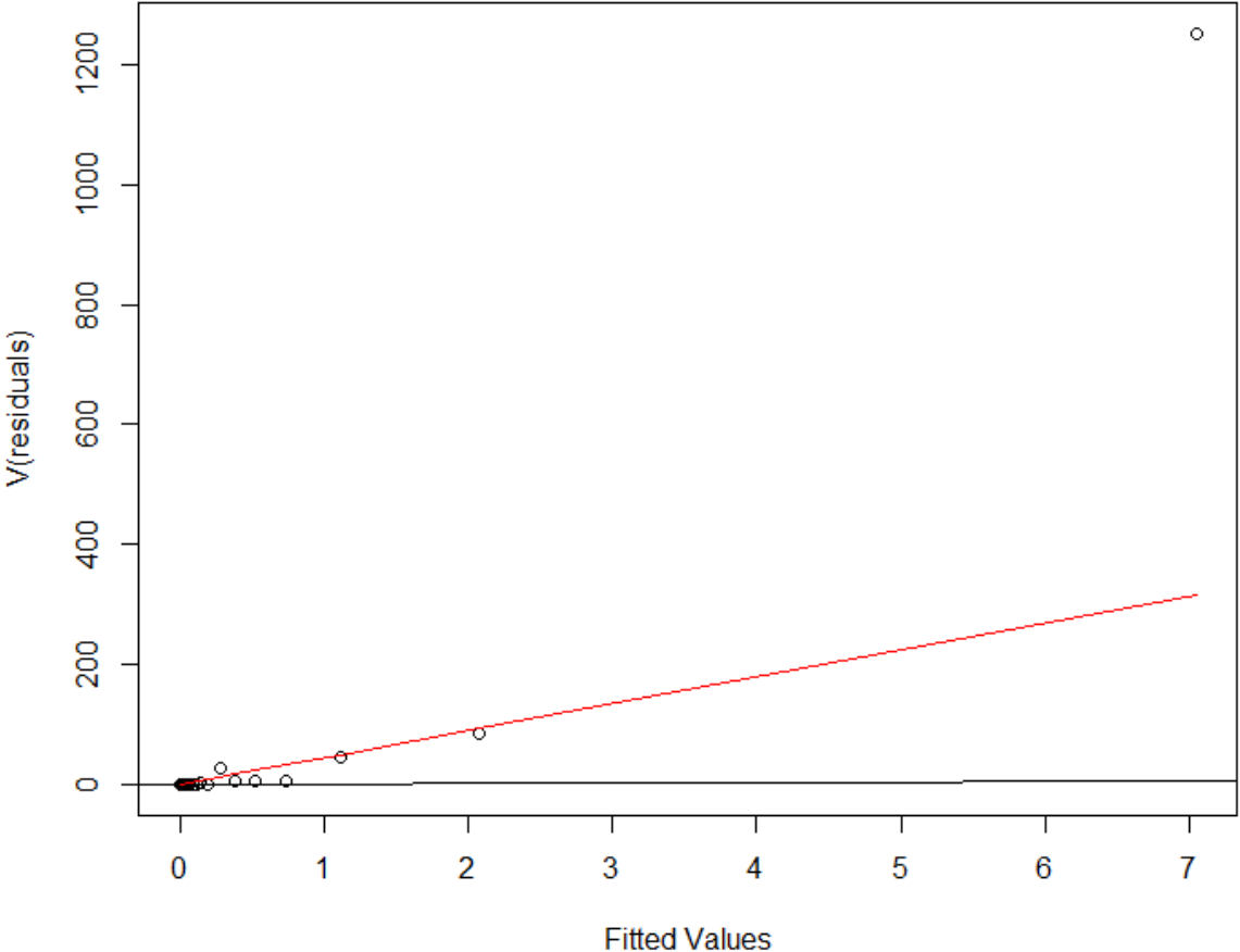
Figure 9: Mean-variance plot for best fitting kittiwake model.
